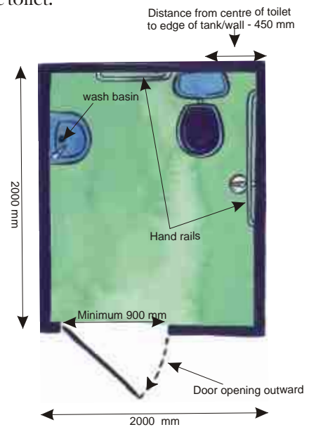
Western-style toilet aerial view
