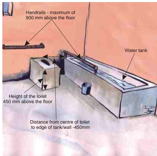
Adapted form of Western-style toilet (front view)
