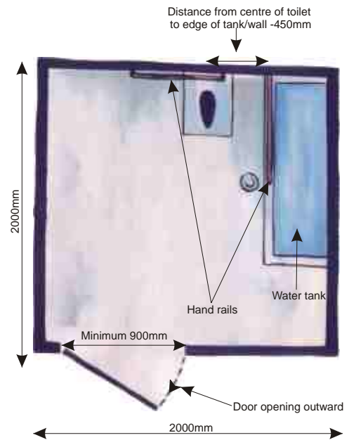
Adapted form of Western-style toilet (aerial view)
